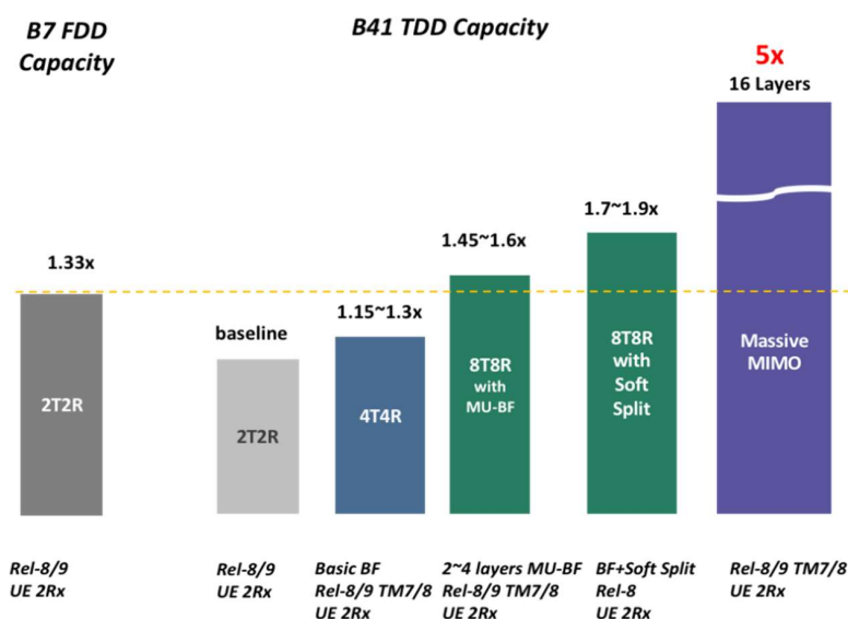
Figure 32: LTE Band 41
