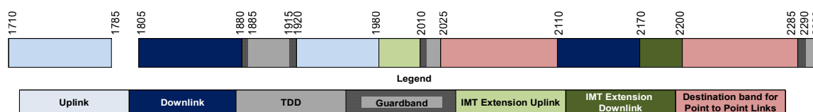
Figure 29: IMT2100-extensions proposal.
