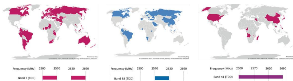
Figure 4: 3GPP LTE spectrum bands in the 2600MHz and countries with launched LTE networks of each band (source: GSA)
