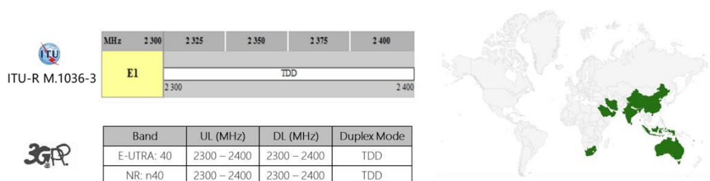
Figure 5: Identification of 2300-2400 MHz frequency band in IMT/3GPP and Countries that use LTE Band 40 (Source: ITU & Huawei)
