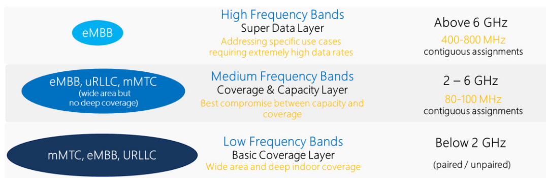
Figure 2: Multi-layer frequencies approach for 5G usage scenarios
