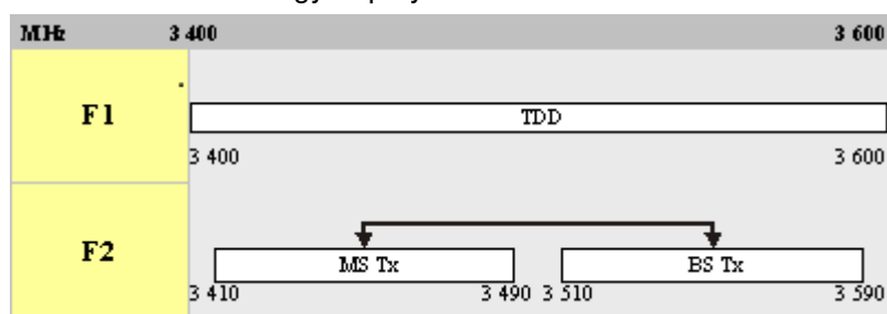
Figure Two 3GPP specified arrangements on 3.5GHz
