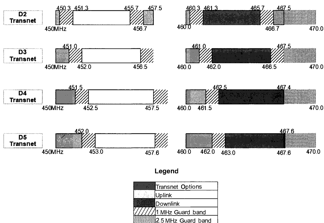
Figure 46: Potential co-existence scenarios for IMT450 with different bandwidths
