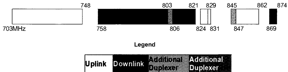
Figure 15: Option1 in 703-876 MHz
