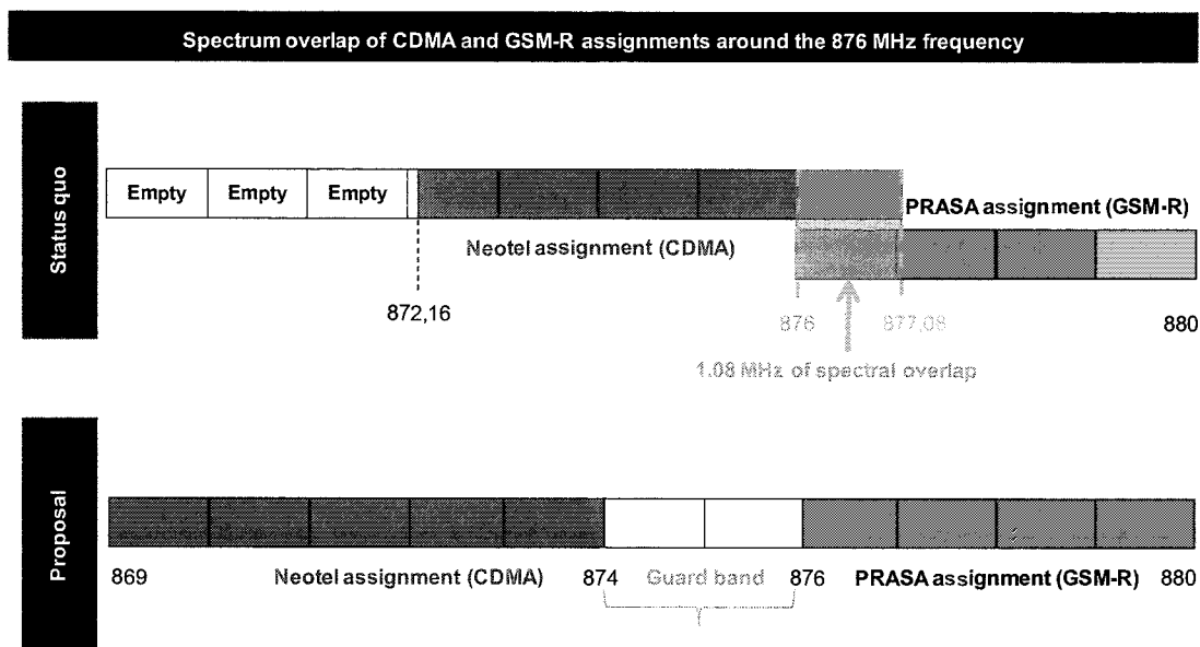
Figure 21: Spectrum overlap of CDMA and GSM-R assignments
