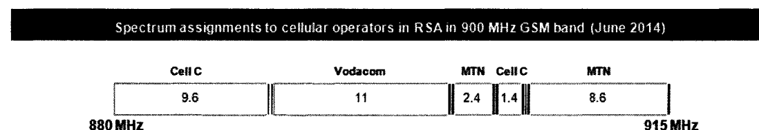
Figure 54: Spectrum assignments to cellular operators in the 900 MHz band
