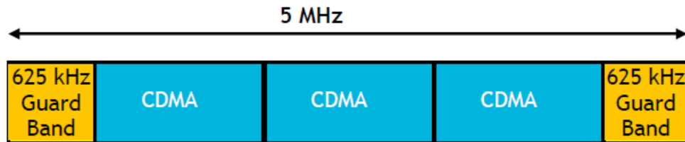
Figure 1: Illustration of 3 CDMA carriers in 5 MHz spectrum block
