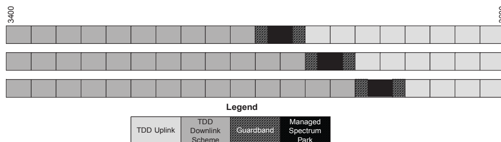
Figure 7: Potential unpaired LTE assignments in 3400-3600 MHz
